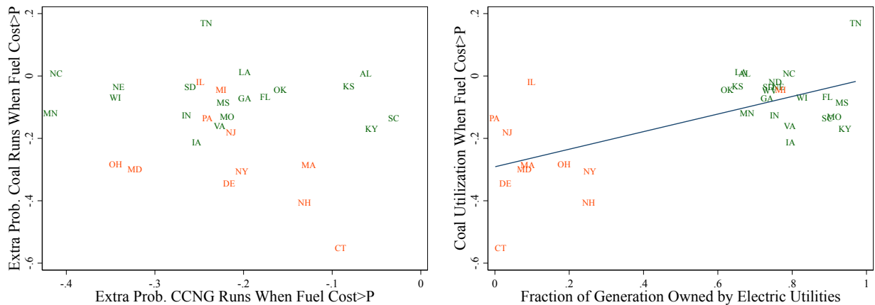
(a) Out-of-Dispatch Order Generation for Coal and CCNG
