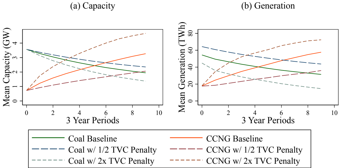
Figure 5: Capacity and Generation for Different TVC Penalties
